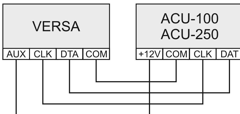
Fig. 12. Connecting the ACU-100 / ACU-250 controller to the control panel.
