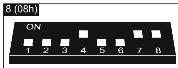
Fig. 14. Setting the DIP-switches in the ACU-100 controller.
