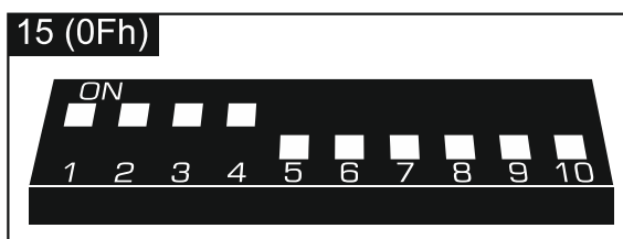
Fig. 18. Setting address, as in the case of the INT-O expander.
