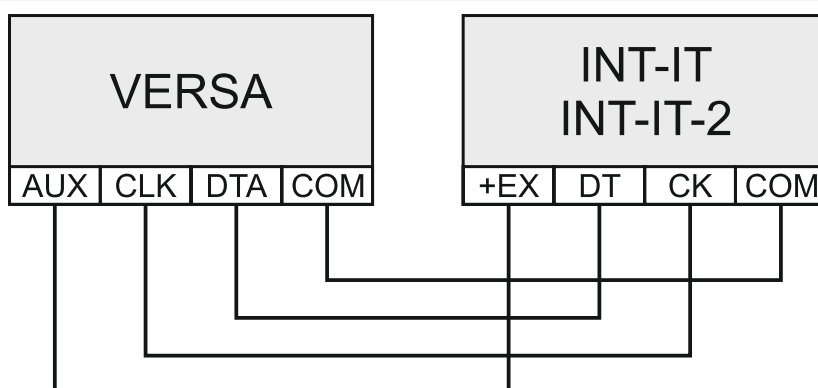
Fig. 19. Connecting the INT-IT / INT-IT-2 module to the control panel.
