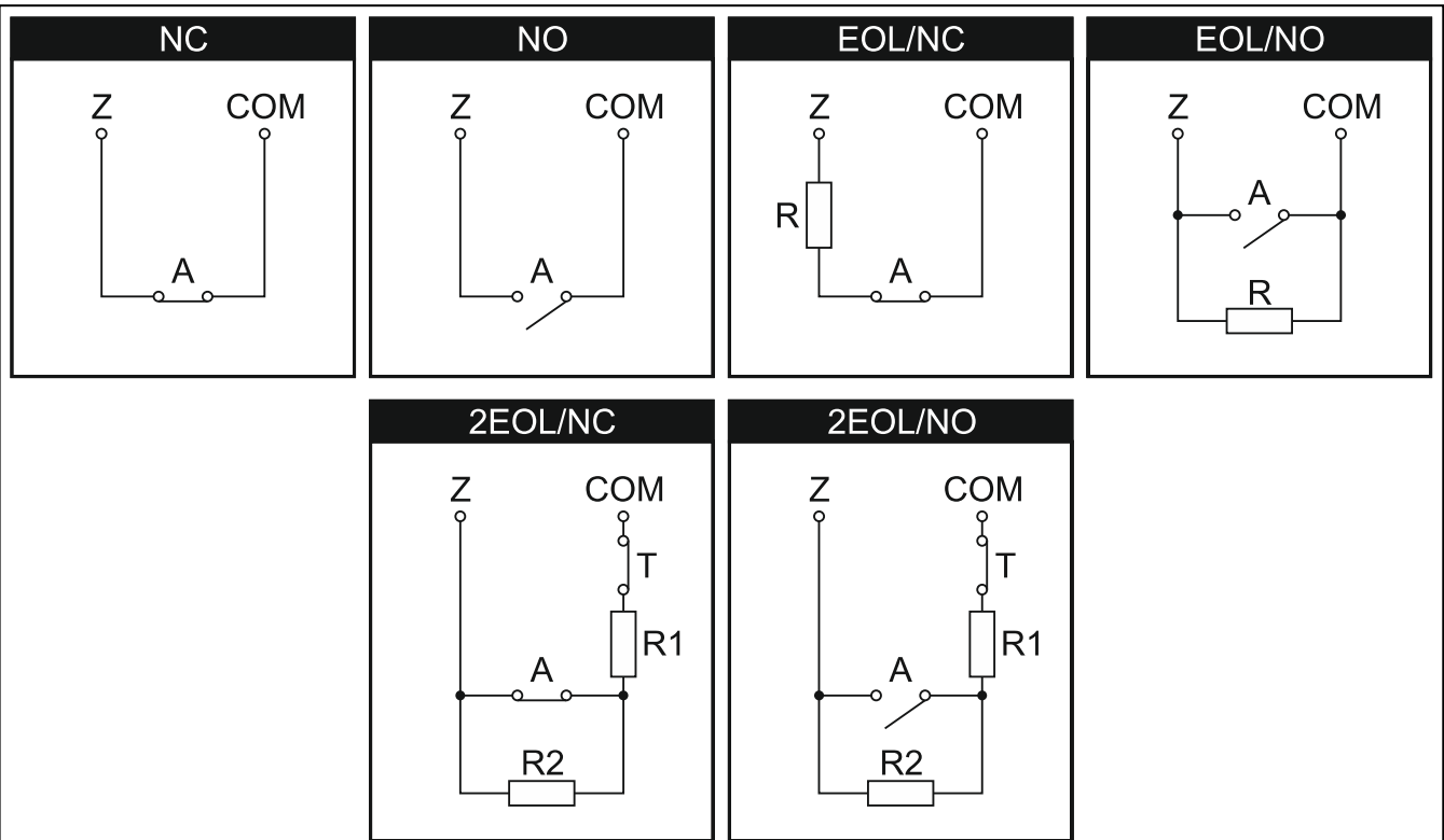
Fig. 22. The ways to connect detectors to zones. The detector outputs are designated with letters: A - alarm, T – tamper. R=R1+R2 .
