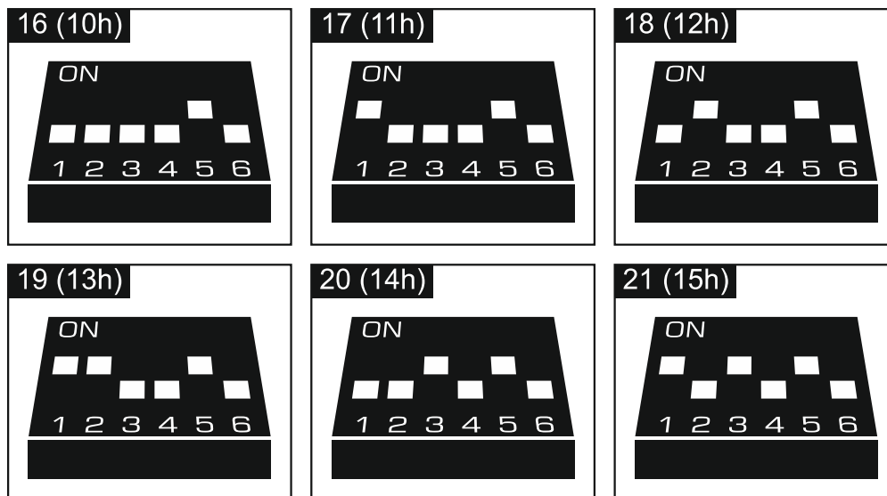
Fig. 20. Setting the address, as in the case of the INT-IT / INT-IT-2 module.
