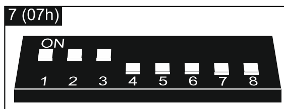
Fig. 9. Setting address in the INT-RX-S / INT-RX expander.
