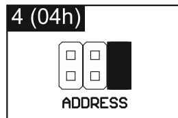
Fig. 7. Setting address in the ETHM-1 Plus module (■ - jumper on; □ - jumper off).
