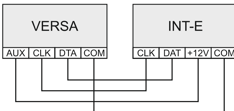
Fig. 15. Connecting the INT-E expander to the control panel.
