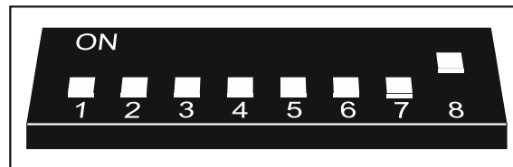
Fig. 13. Setting the DIP-switches in the ACU-120 / ACU-270 controller.
