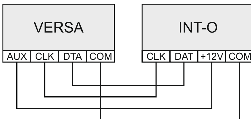
Fig. 17. Connecting the INT-O expander to the control panel.
