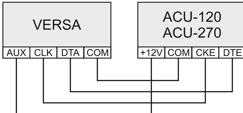
Fig. 11. Connecting the ACU-120 / ACU-270 controller to the control panel.
