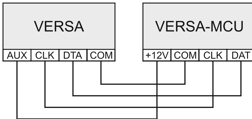
Fig. 10. Connecting the VERSA-MCU controller to the control panel.
