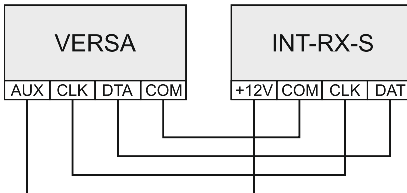
Fig. 8. Connecting the INT-RX-S expander to the control panel.
