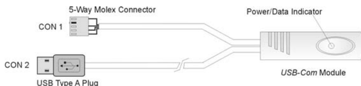
Figure 1. USB-Com Connectors
