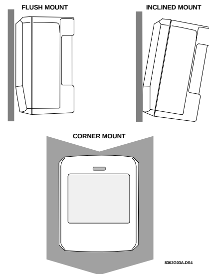
Figure 15. Wall Mount Options: use the inclined position for surface or corner mounting with the standard lens. Use the flush position for surface or corner mounting with the animal alley lens.
