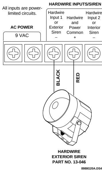
Figure 2. Exterior Siren Control Panel Connections
