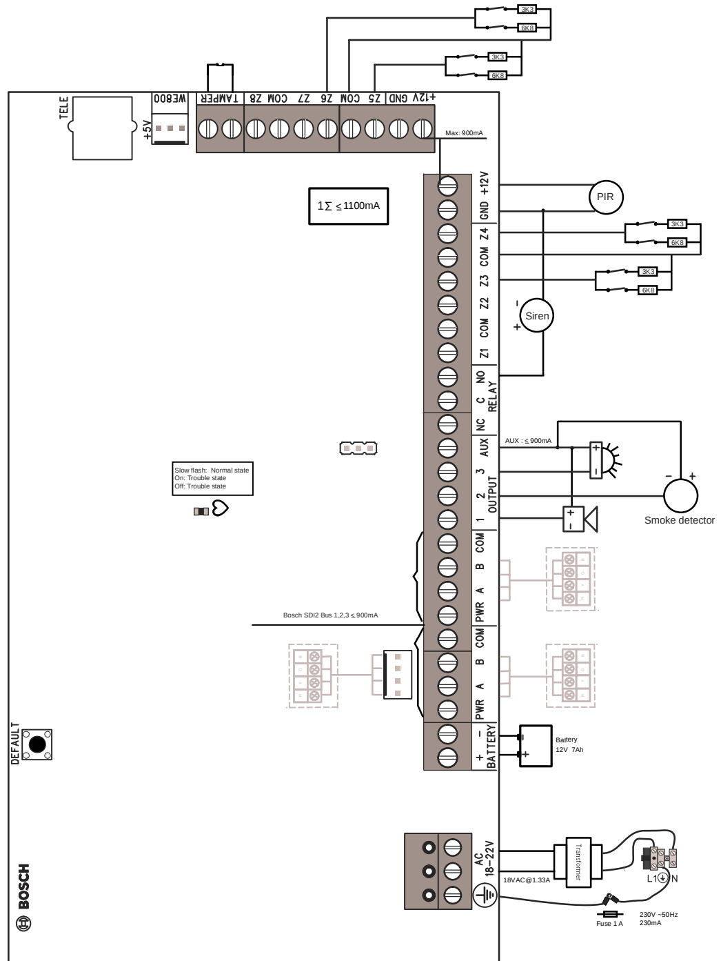
Figure 5.1: Wiring Diagram
